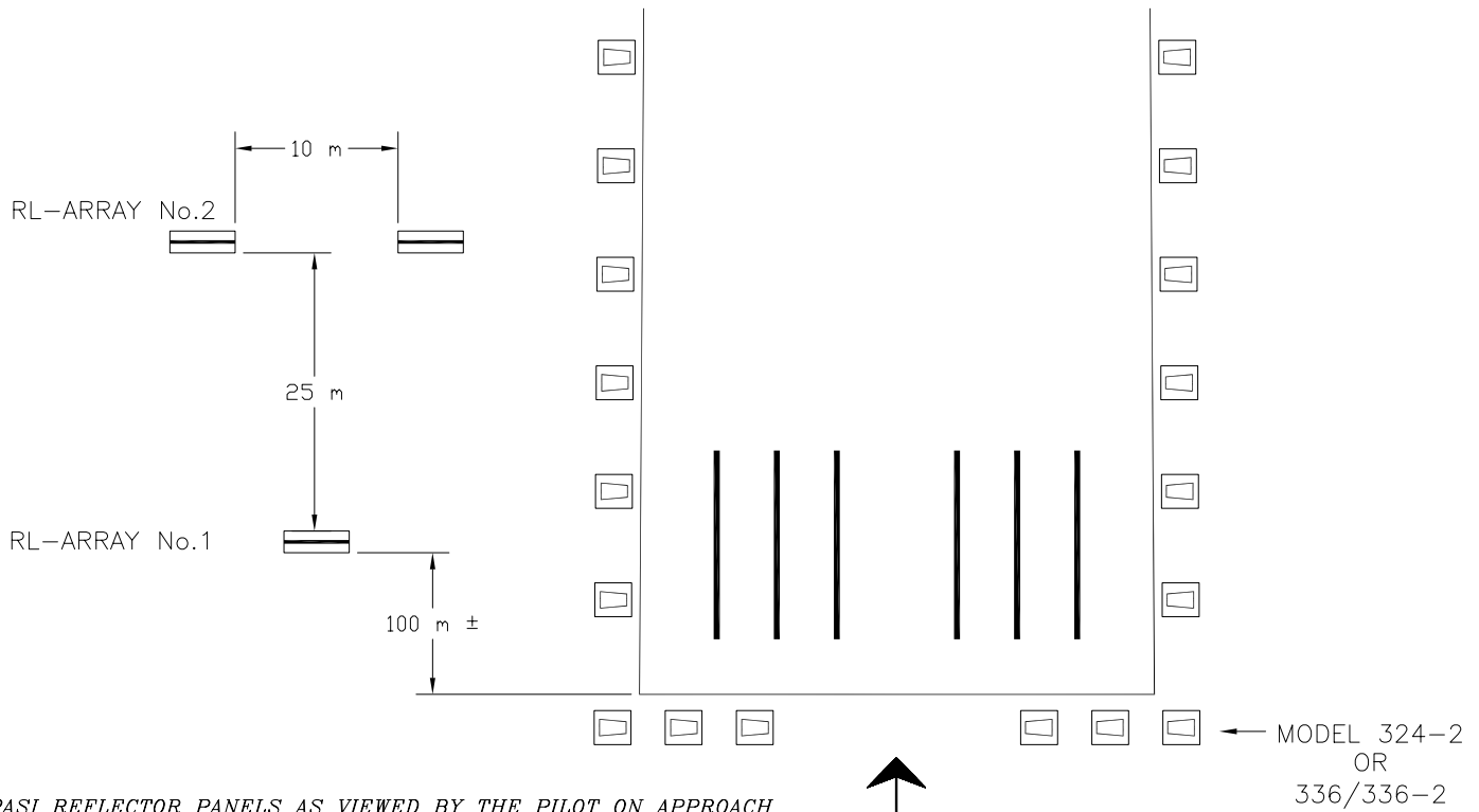
PASI REFLECTOR PANELS AS VIEWED BY THE PILOT ON APPROACH
